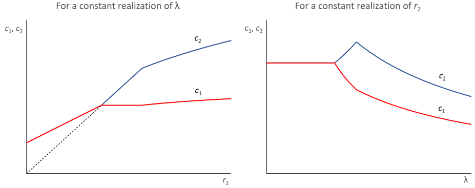
Figure 1: Optimal consumption
